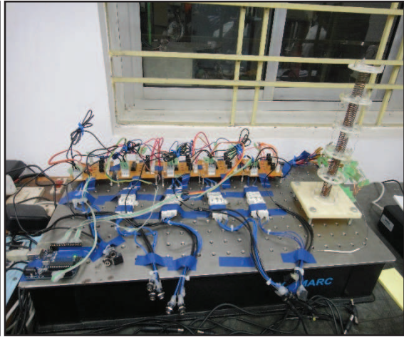
Flexible Manipulator
